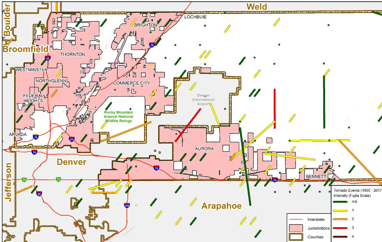
Figure 4-45 Tornado Events in West Adams County 1950-2017
