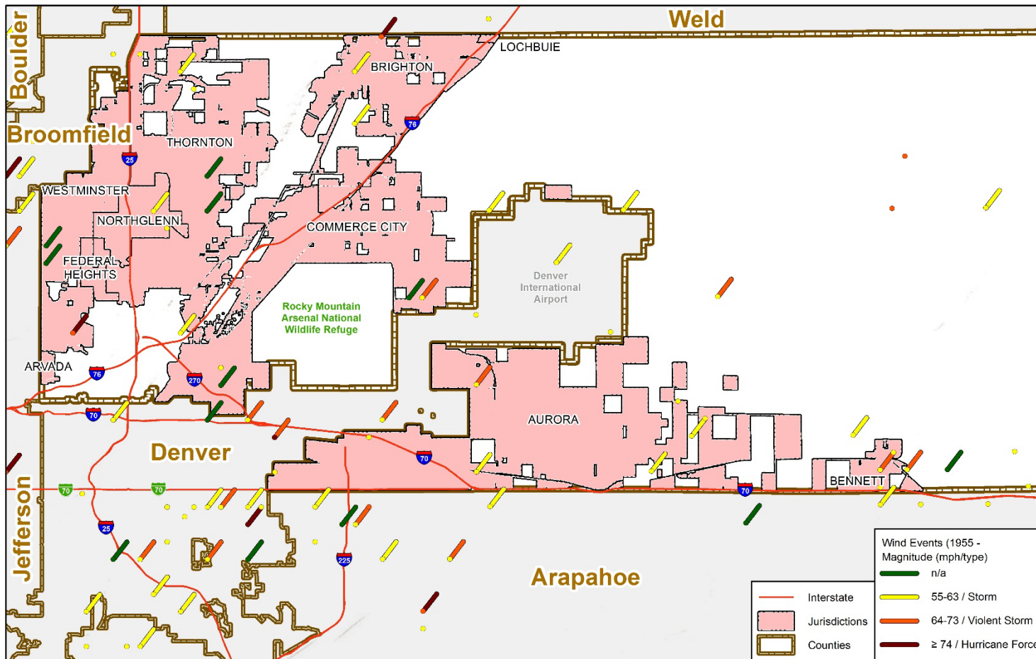
Figure 4-47 Wind Events in West Adams County 1955-2017
