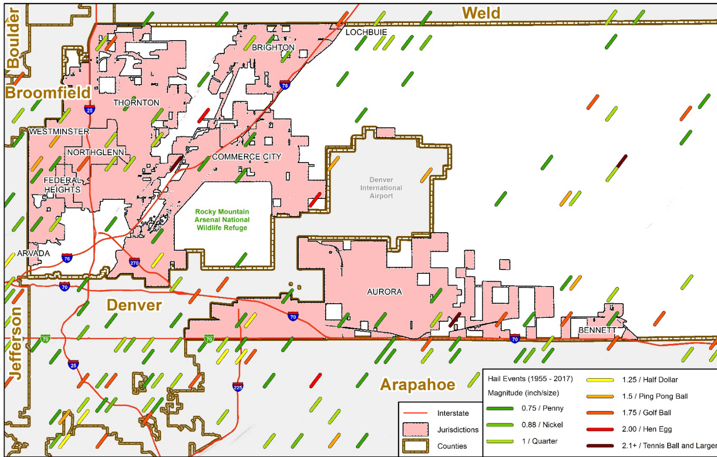
Figure 4-41 NOAA Hail Events in West Adams County, 1955-2017
