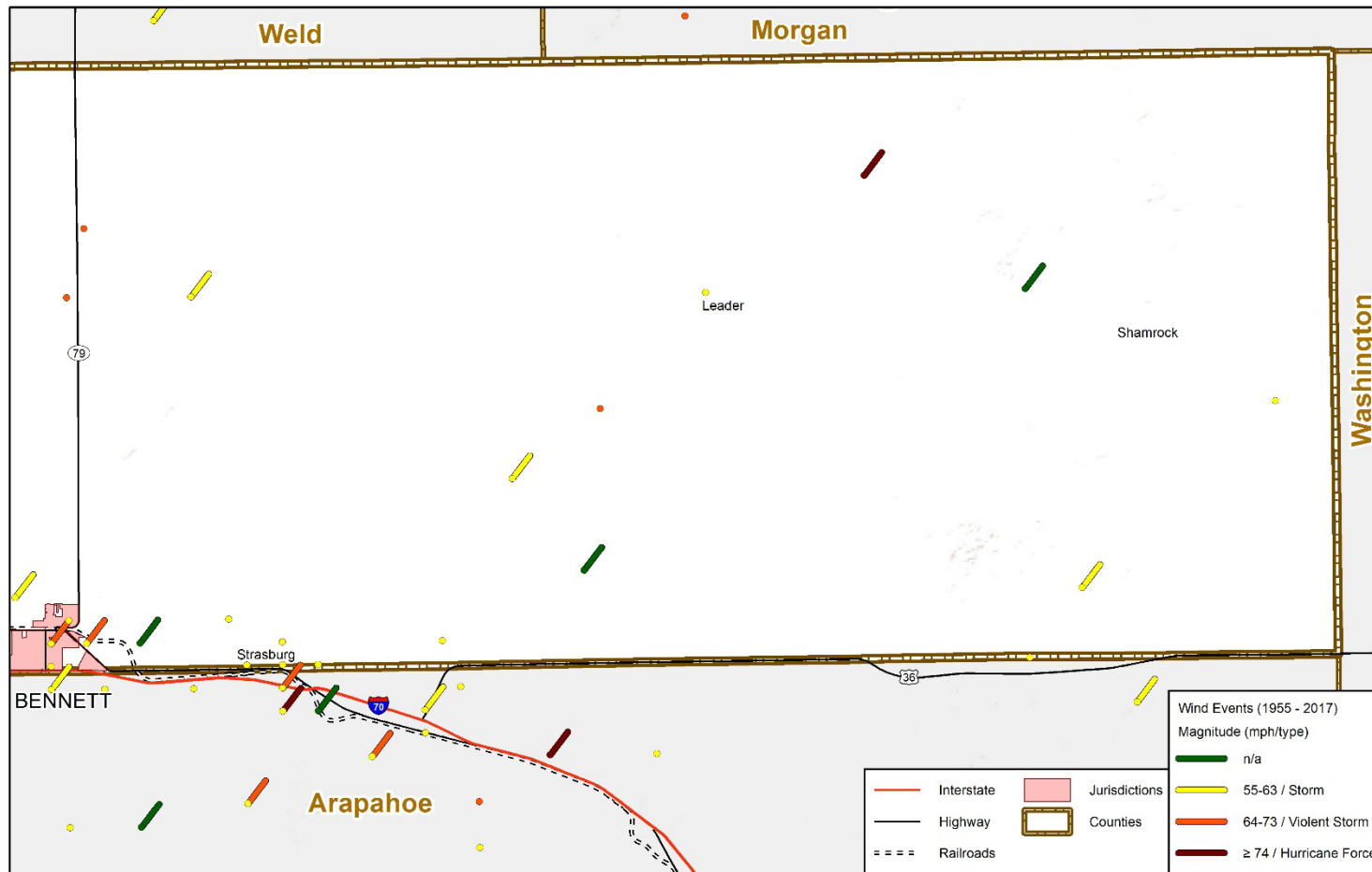
Figure 4-48 Wind Events in East Adams County 1955-2017
