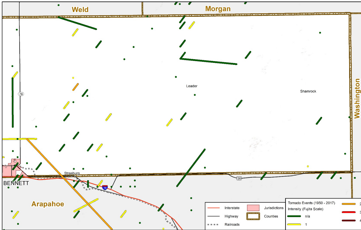
Figure 4-46 Tornado Events in East Adams County 1950-2017
