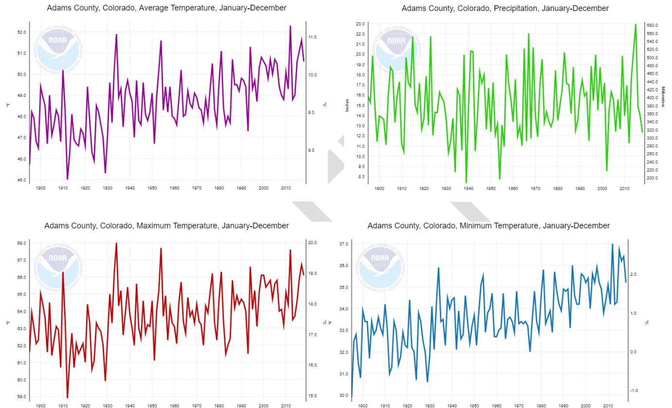
Figure 2-15 Temperature and Precipitation Trends for Adams county, 1890-2019
