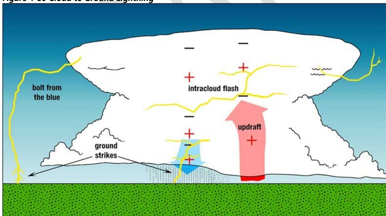
Figure 4-39 Cloud to Ground Lightning
