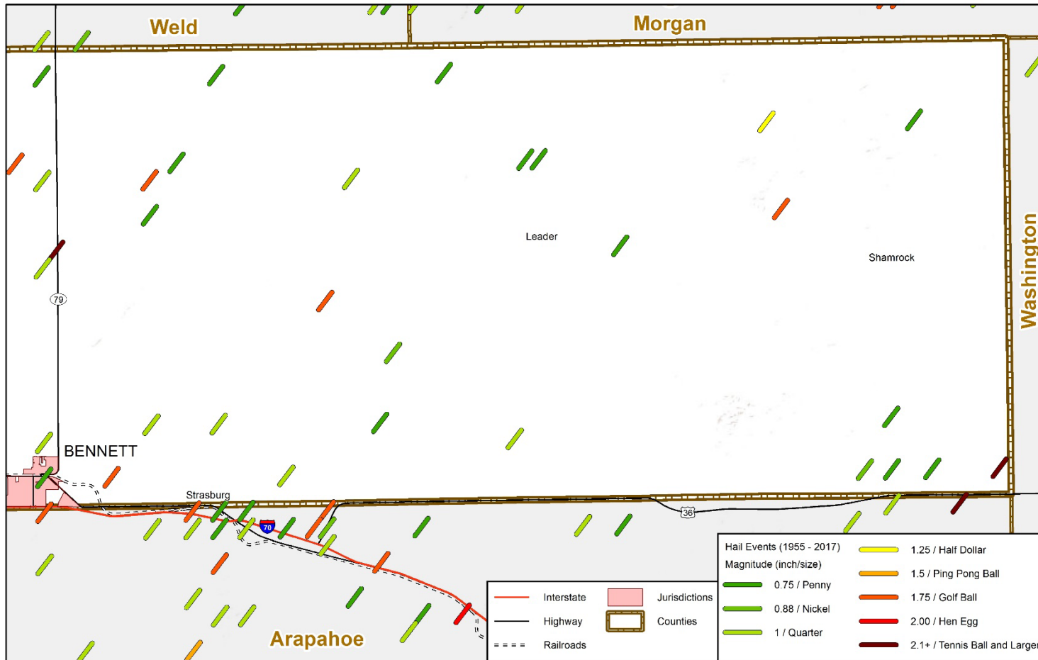
Figure 4-42 NOAA Hail Events in East Adams County, 1955-2017
